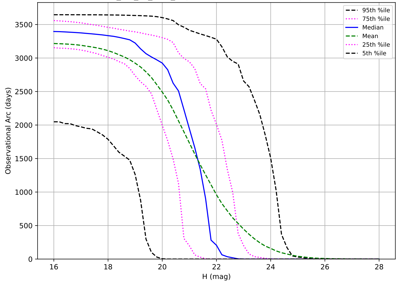
mw_roll_all_v3.3_10yrs: Observational Arc Length PHA
