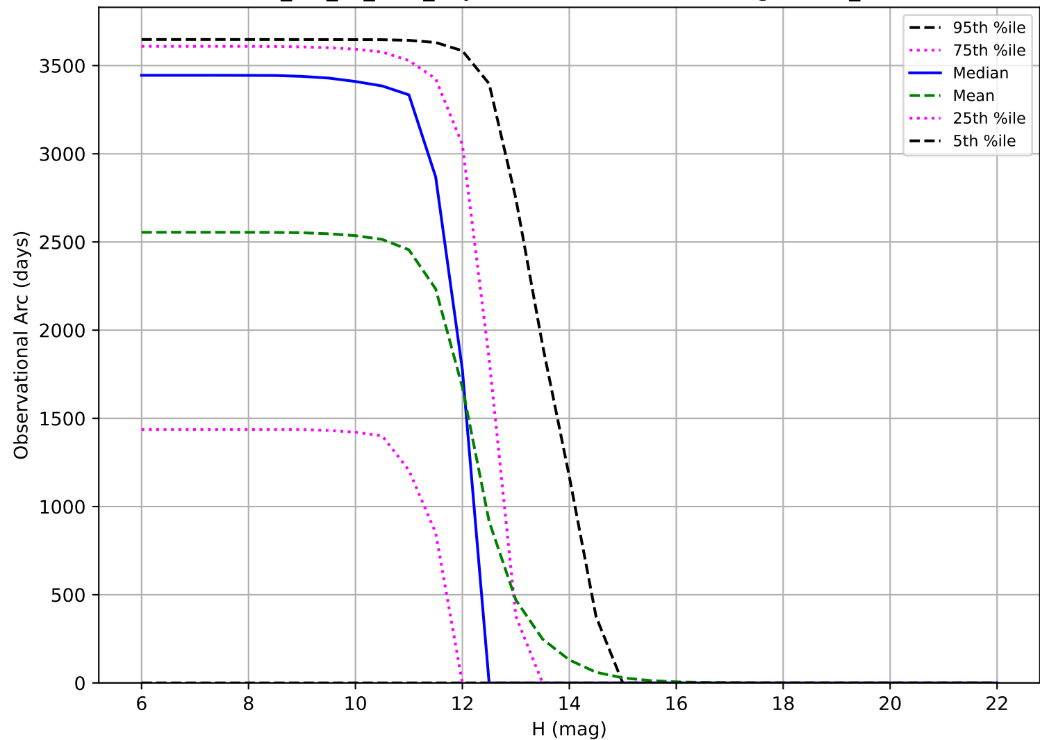
mw_roll_all_v3.3_10yrs: Observational Arc Length OCC_r20
