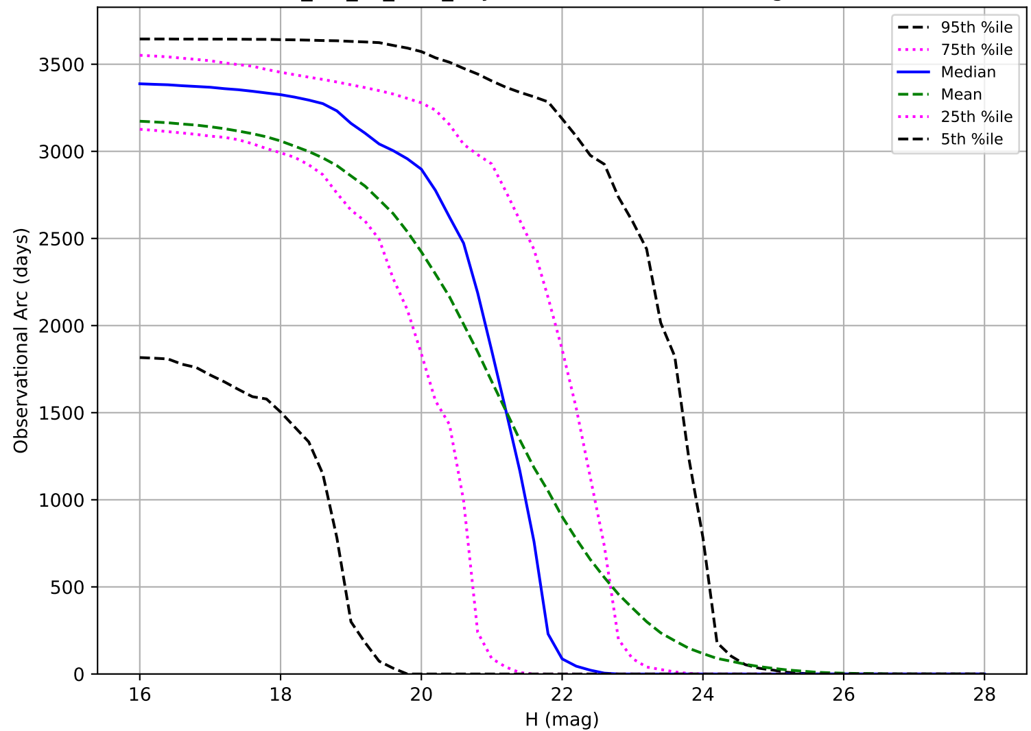
mw_roll_all_v3.3_10yrs: Observational Arc Length NEO
