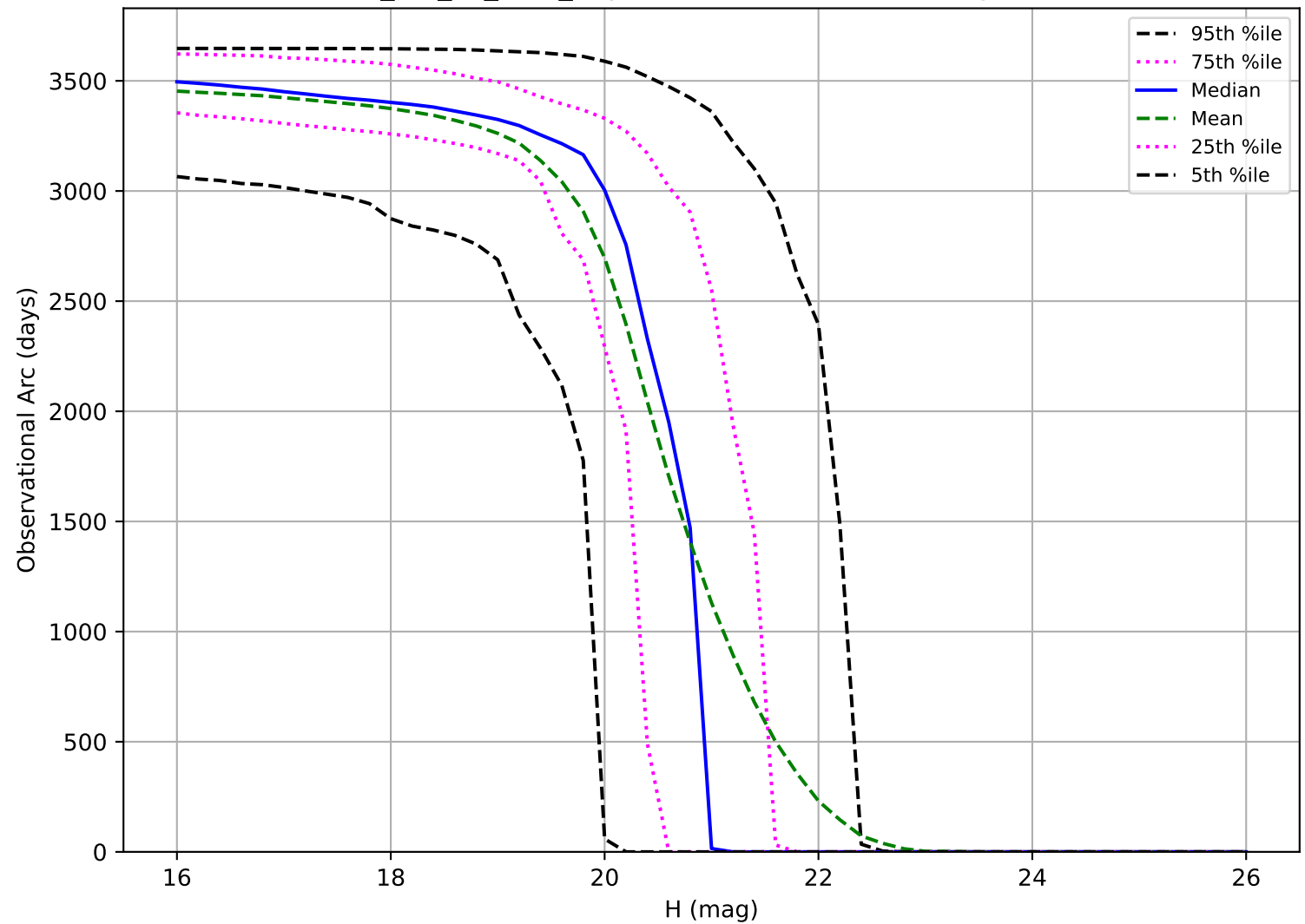
mw_roll_all_v3.3_10yrs: Observational Arc Length MBA
