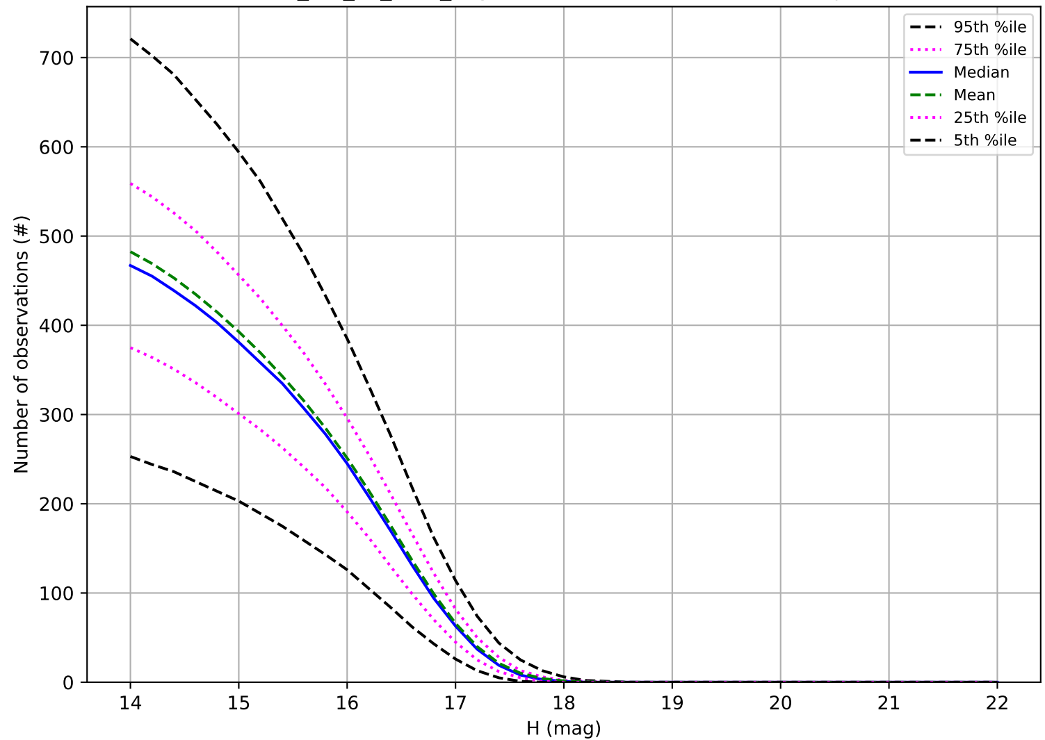
mw_roll_all_v3.3_10yrs: Number of observations Trojan
