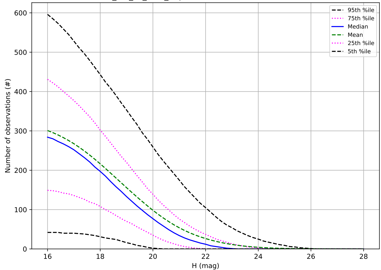
mw_roll_all_v3.3_10yrs: Number of observations PHA
