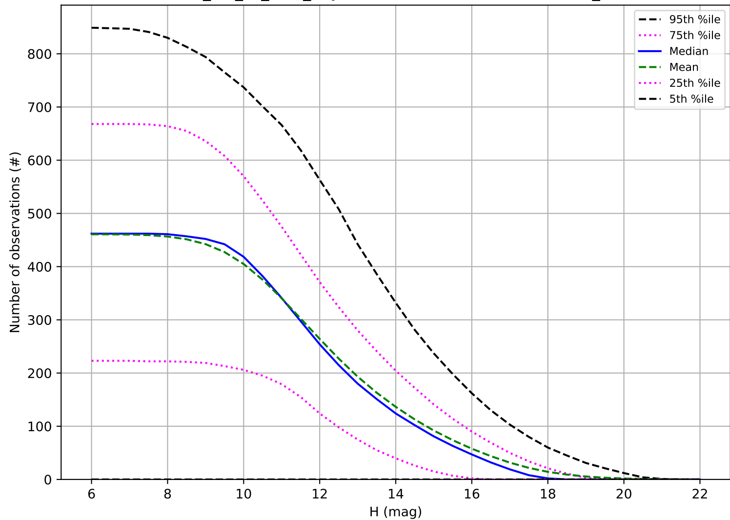
mw_roll_all_v3.3_10yrs: Number of observations OCC_r5
