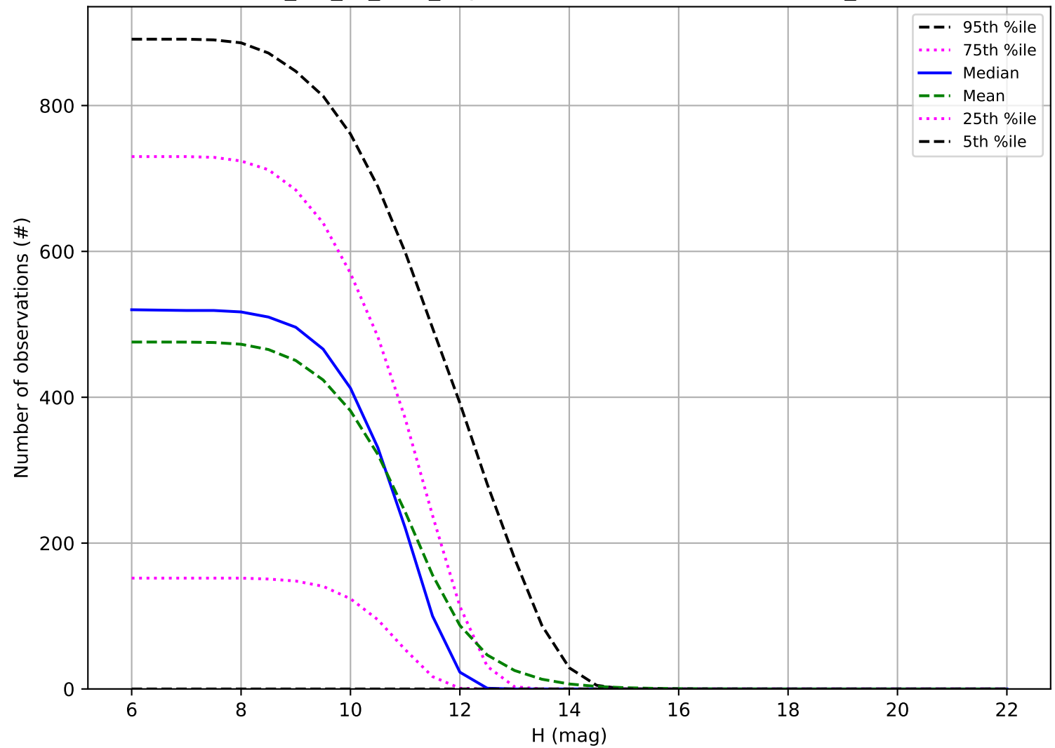
mw_roll_all_v3.3_10yrs: Number of observations OCC_r20
