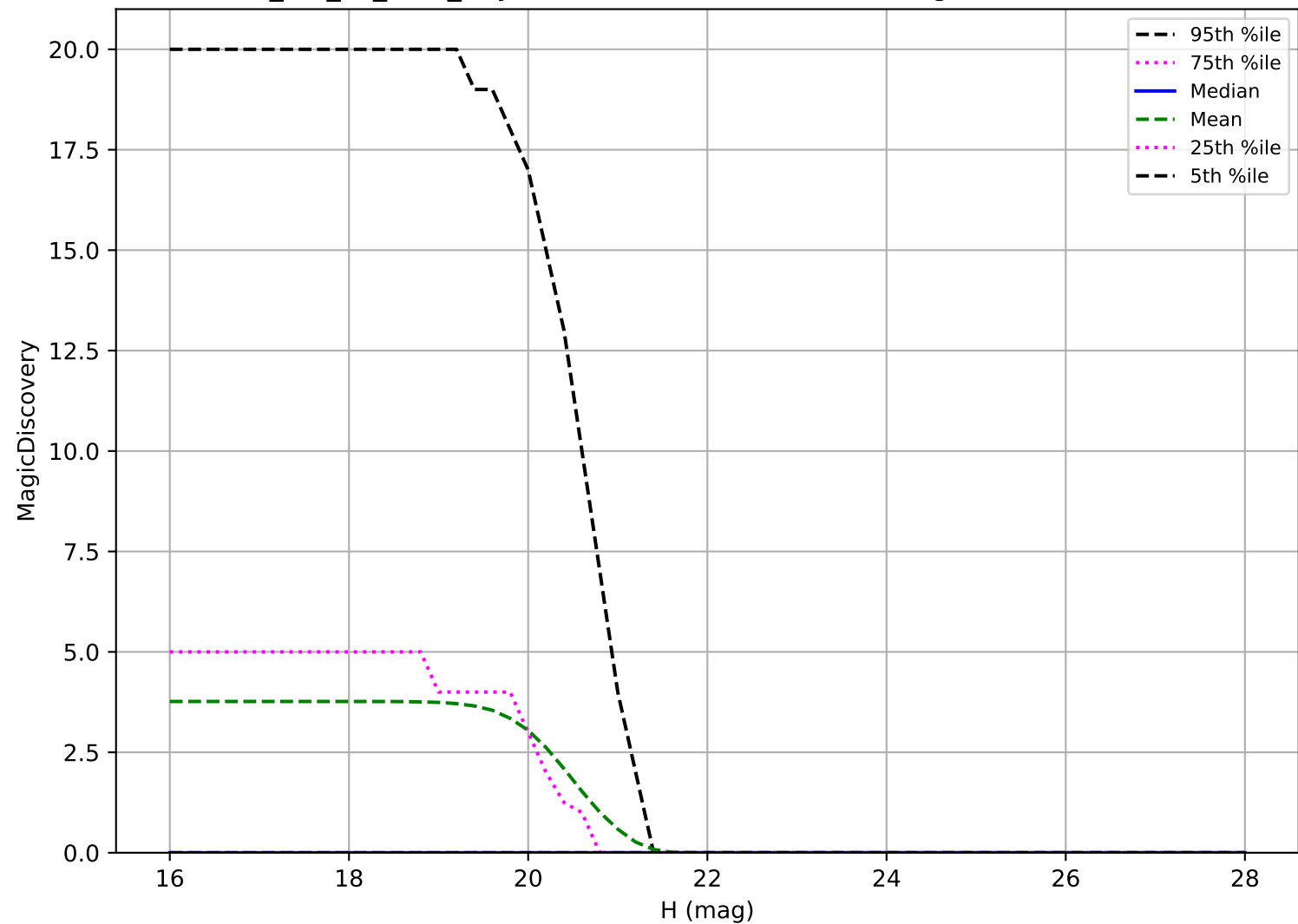
mw_roll_all_v3.3_10yrs: Vatira 6 detections in 60 nights detection loss
