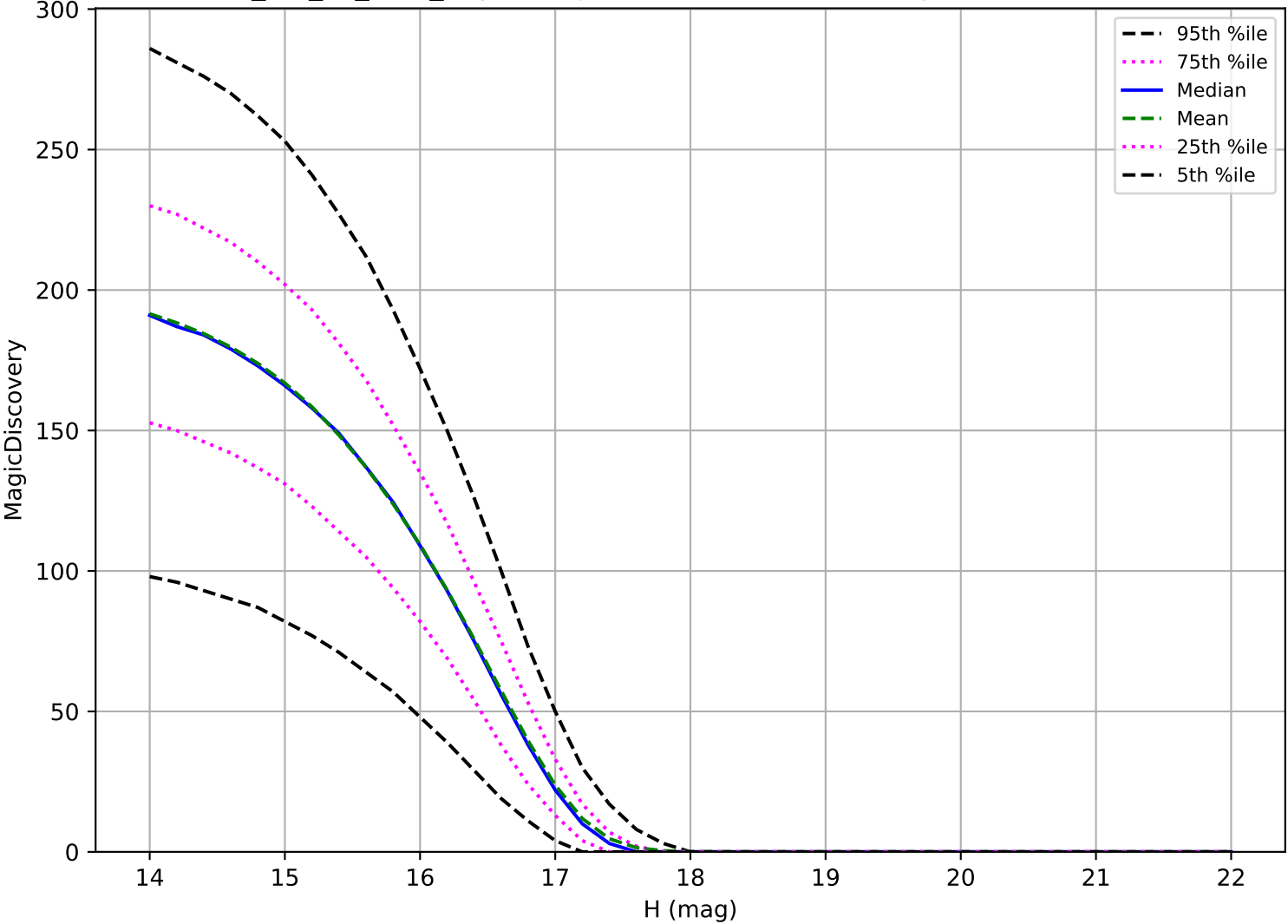
mw_roll_all_v3.3_10yrs: Trojan 6 detections in 60 nights detection loss
