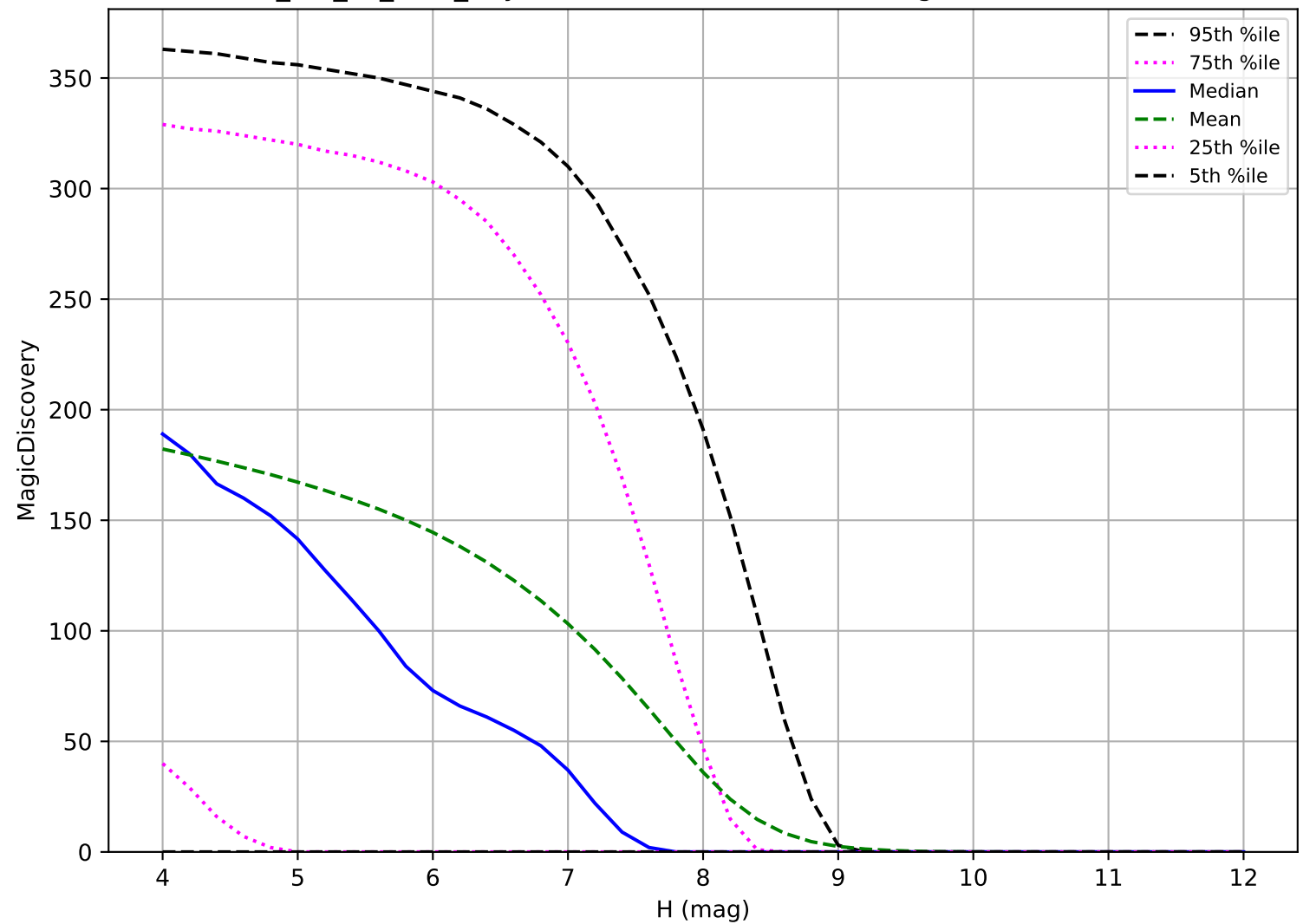
mw_roll_all_v3.3_10yrs: TNO 6 detections in 60 nights detection loss
