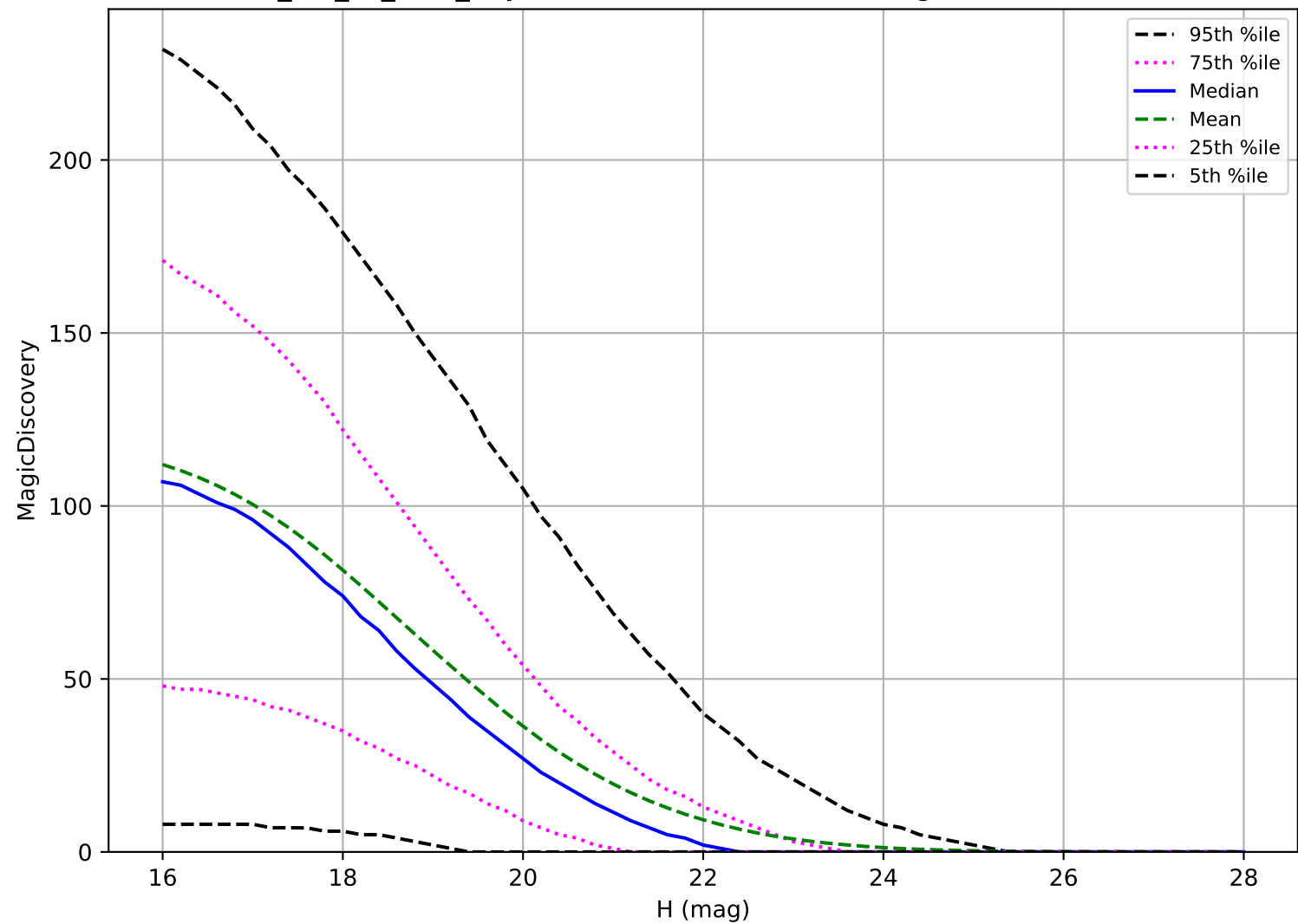
mw_roll_all_v3.3_10yrs: PHA 6 detections in 60 nights detection loss
