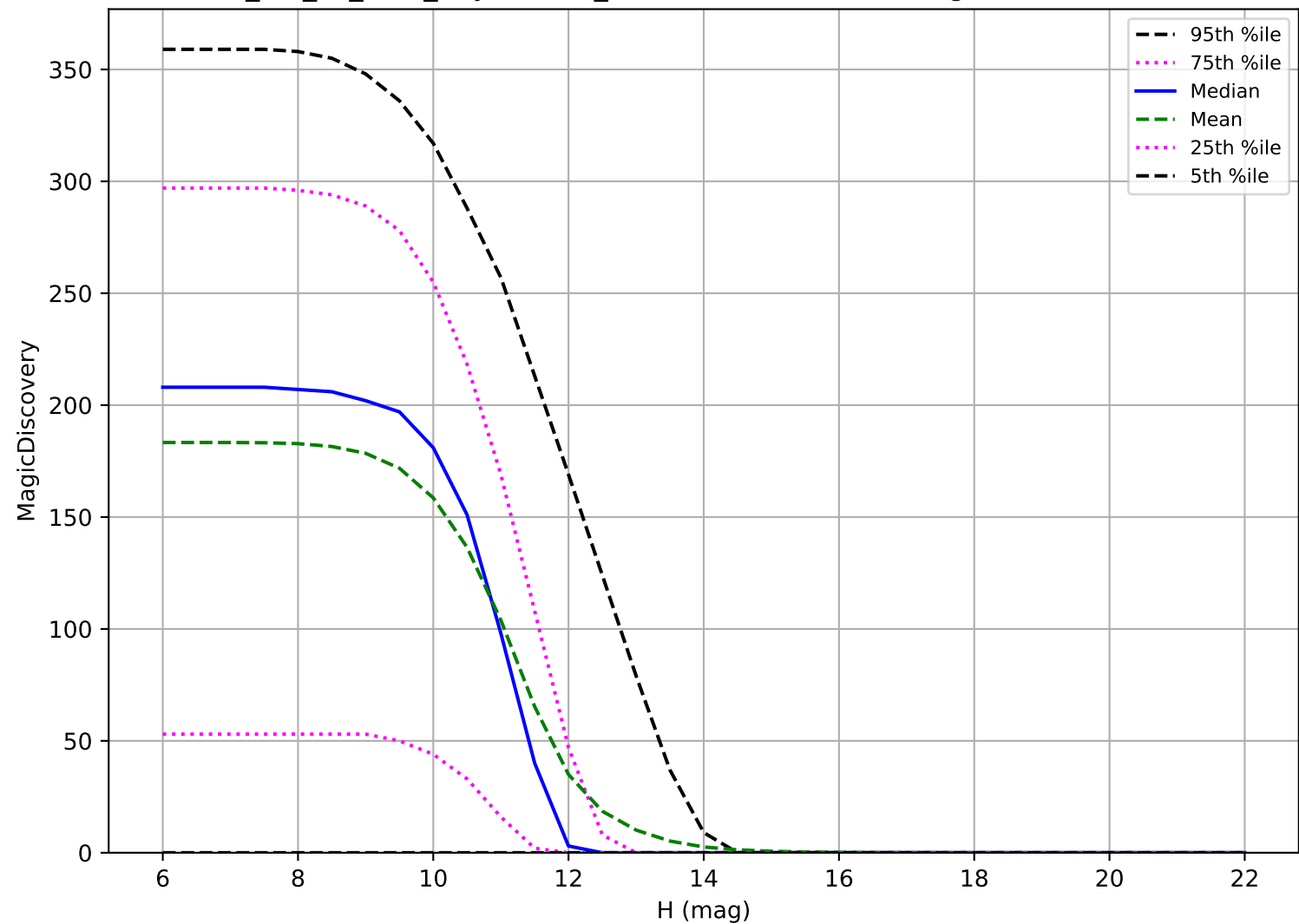
mw_roll_all_v3.3_10yrs: OCC_r20 6 detections in 60 nights detection loss
