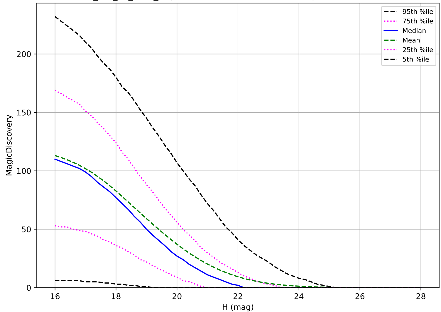
mw_roll_all_v3.3_10yrs: NEO 6 detections in 60 nights detection loss
