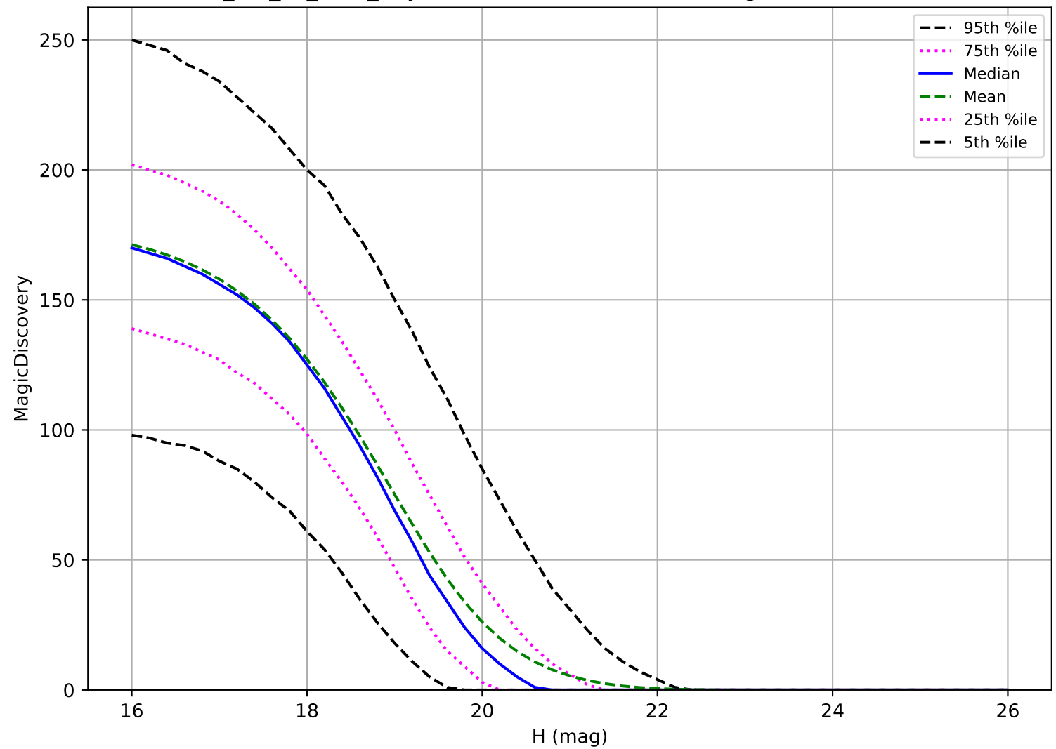
mw_roll_all_v3.3_10yrs: MBA 6 detections in 60 nights detection loss
