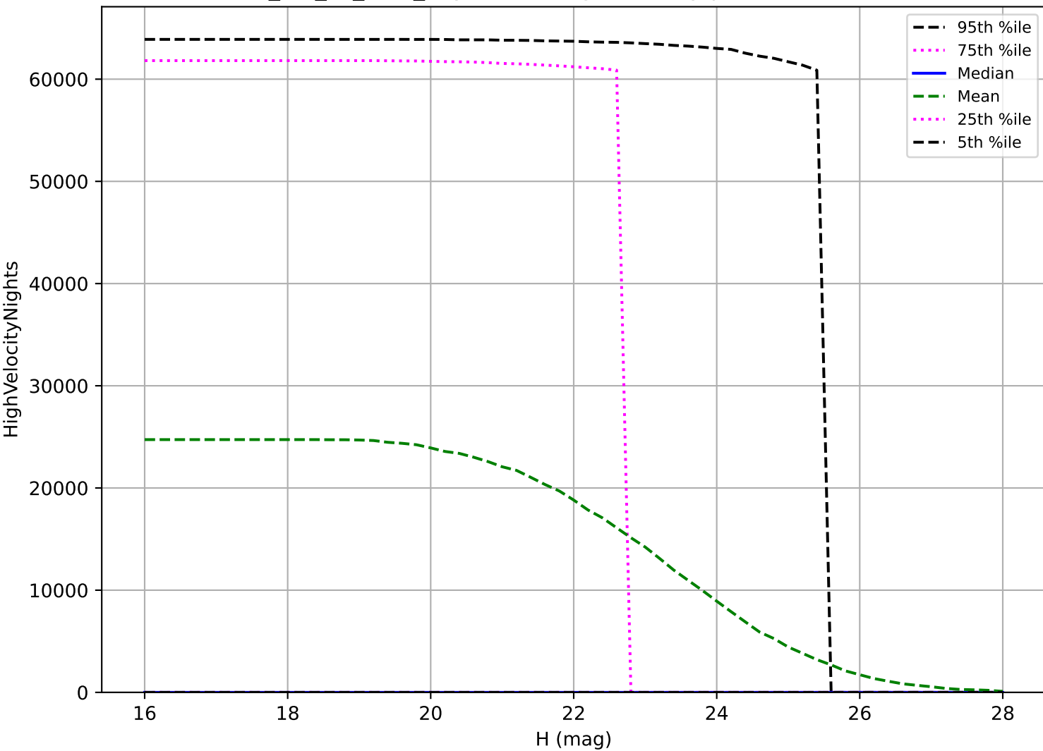
mw_roll_all_v3.3_10yrs: PHA High velocity pair detection loss
