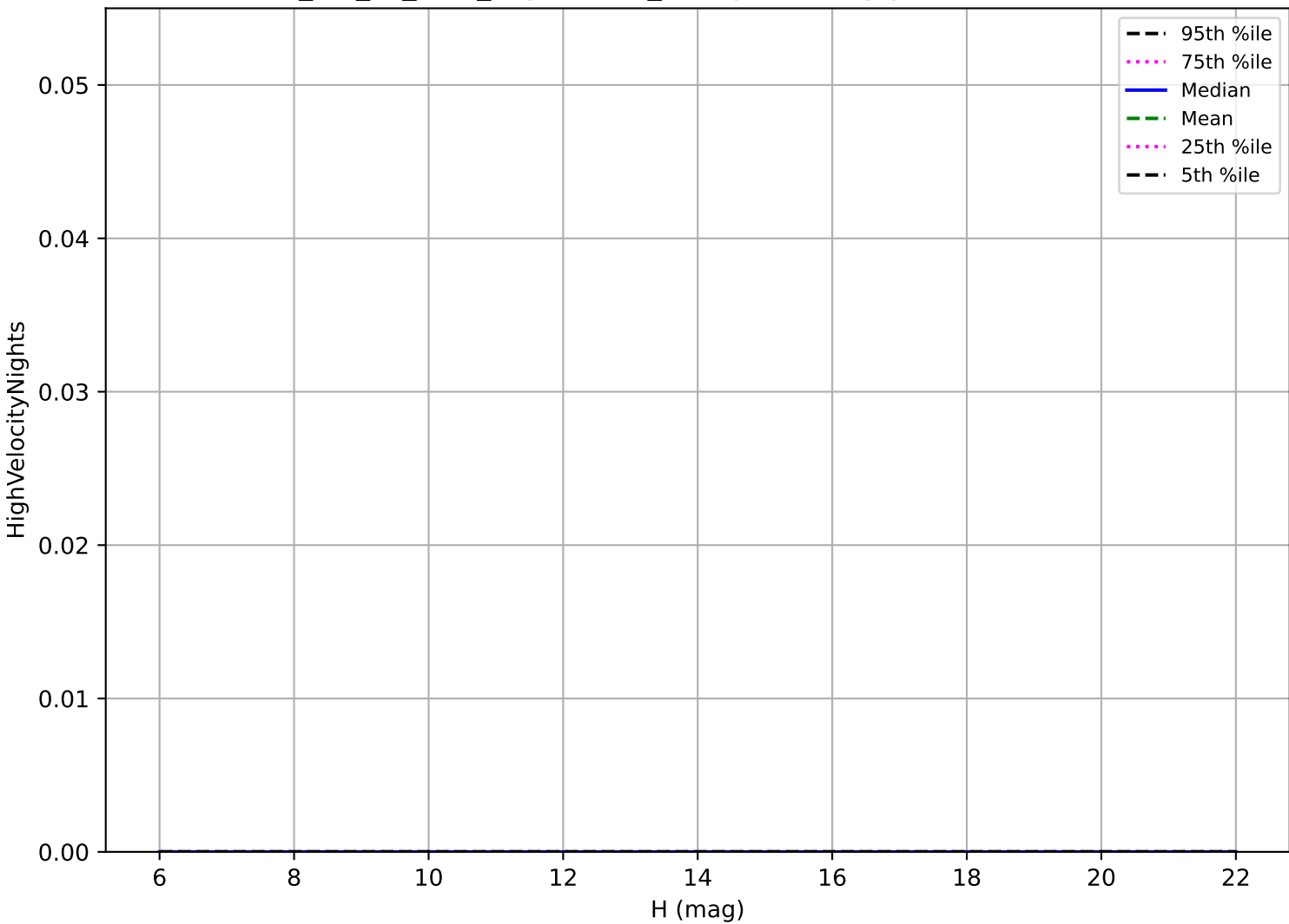
mw_roll_all_v3.3_10yrs: OCC_r5 High velocity pair detection loss
