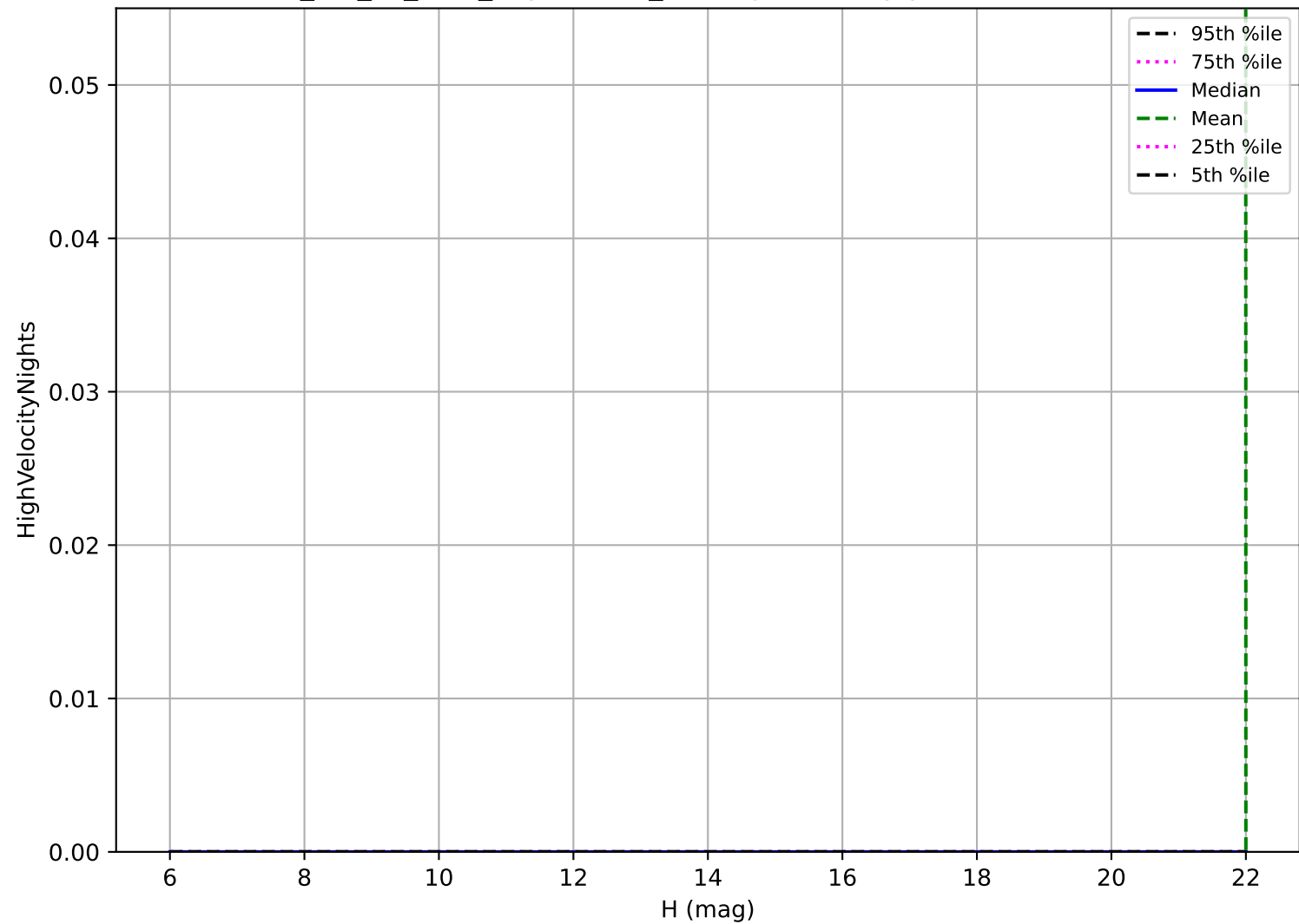
mw_roll_all_v3.3_10yrs: OCC_r20 High velocity pair detection loss
