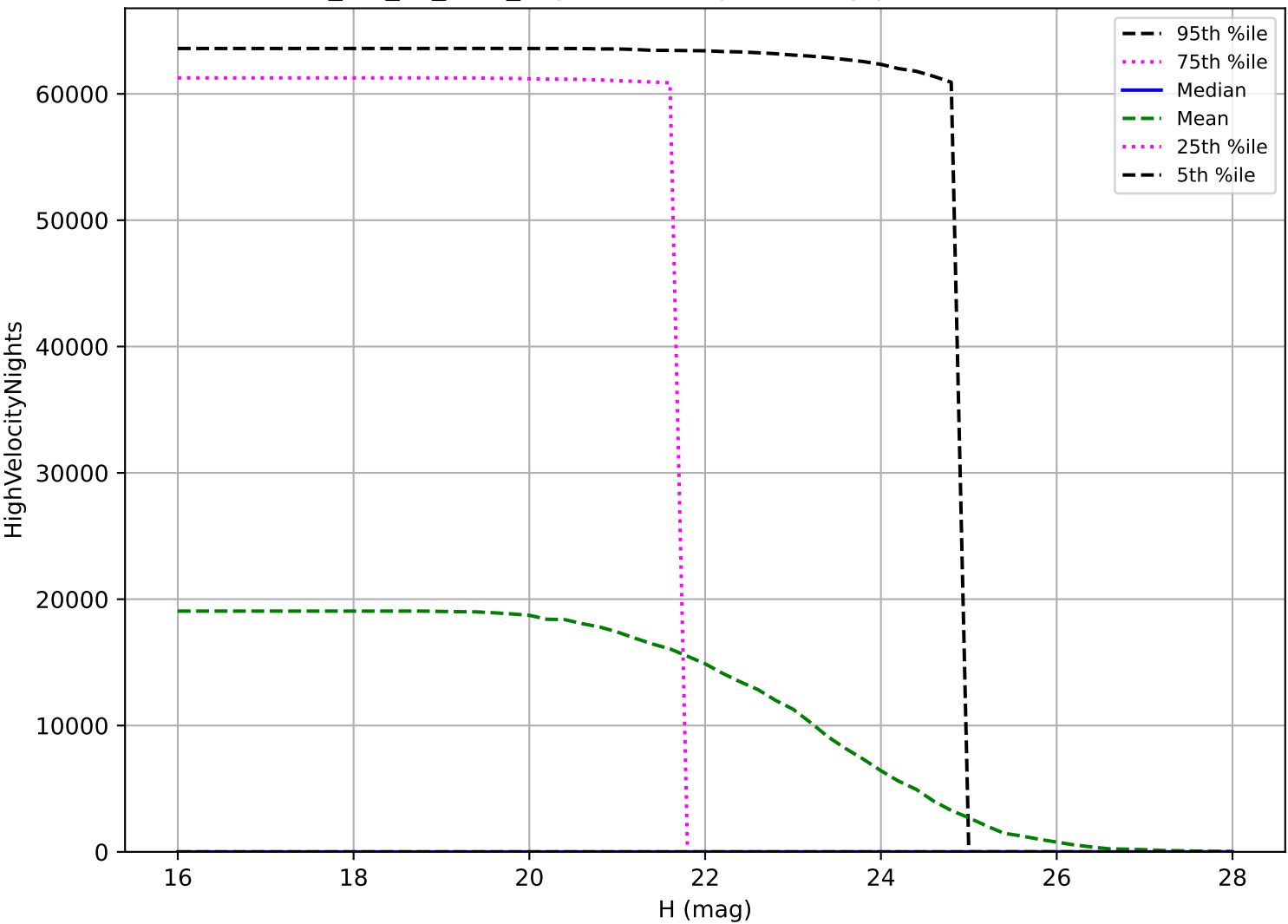
mw_roll_all_v3.3_10yrs: NEO High velocity pair detection loss
