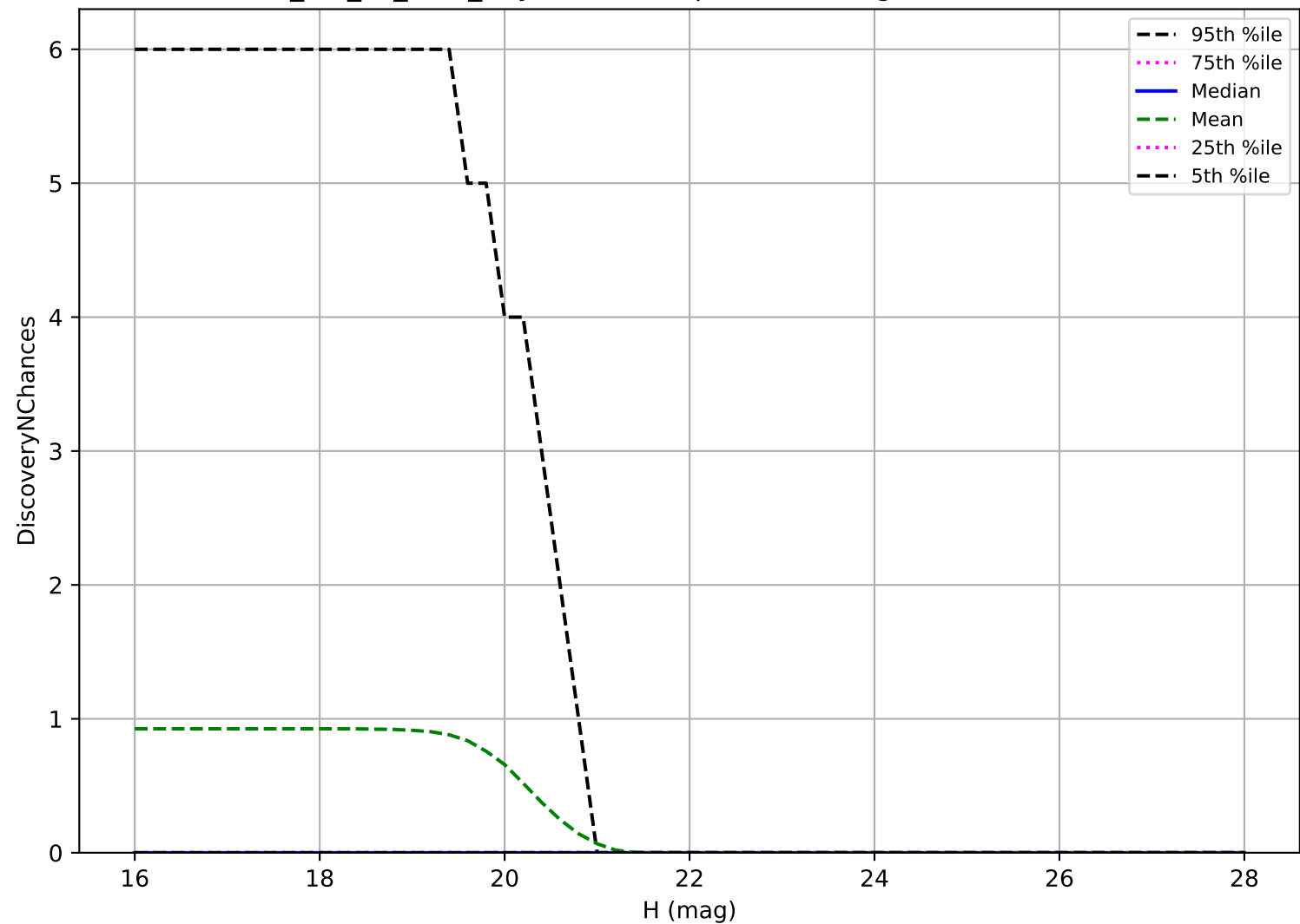
mw_roll_all_v3.3_10yrs: Vatira 3 pairs in 15 nights detection loss
