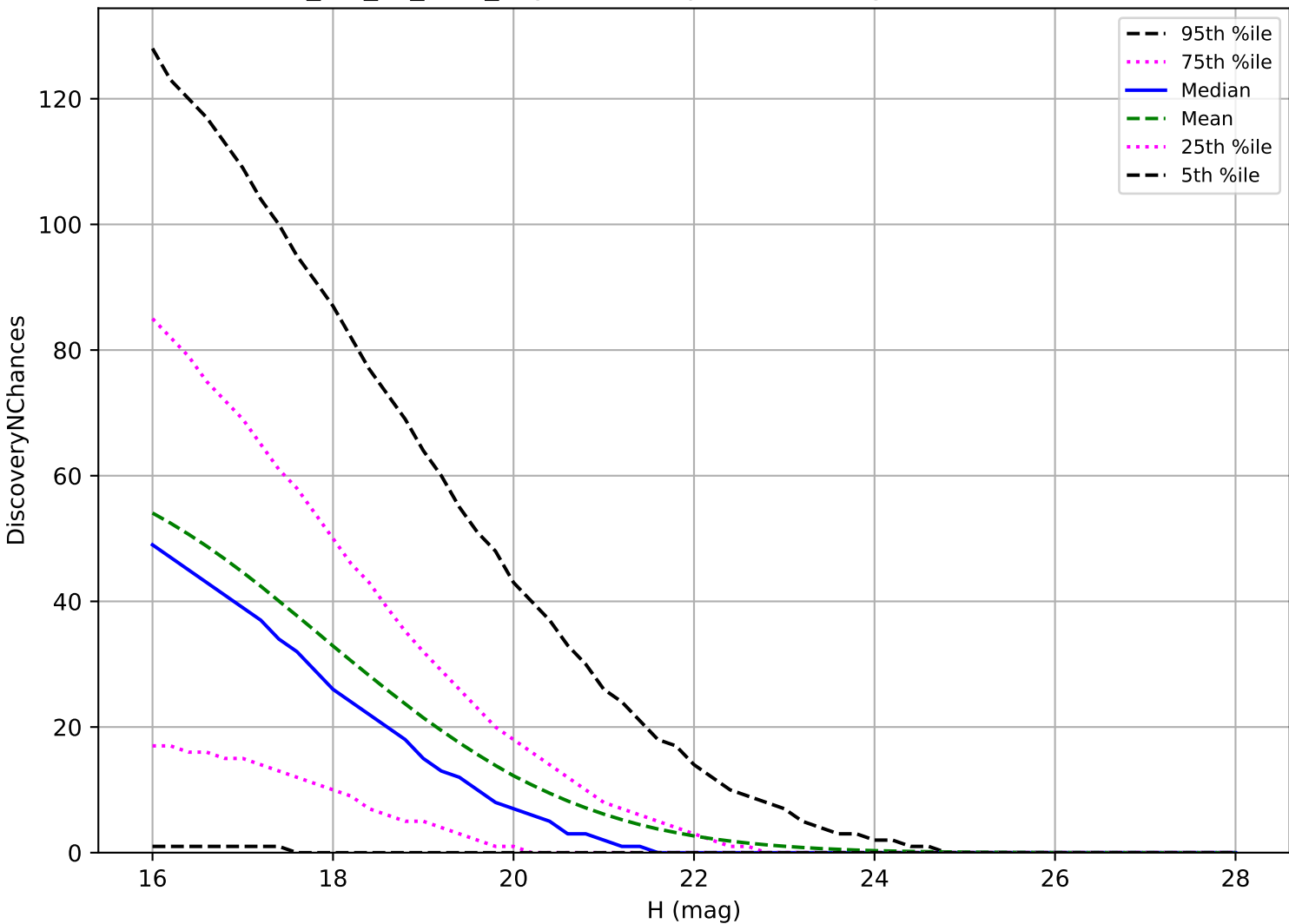
mw_roll_all_v3.3_10yrs: PHA 3 pairs in 15 nights detection loss
