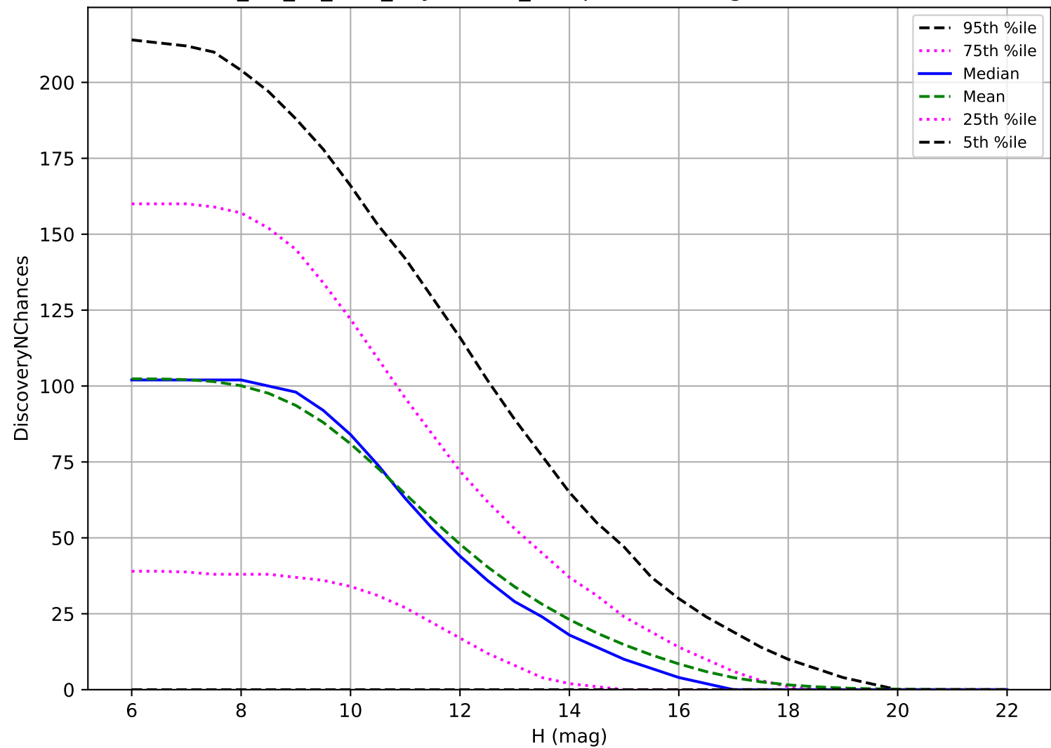
mw_roll_all_v3.3_10yrs: OCC_r5 3 pairs in 15 nights detection loss
