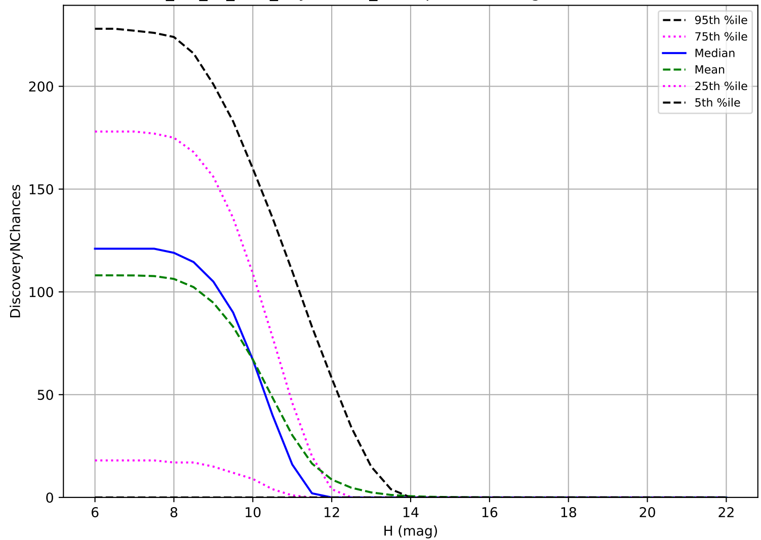
mw_roll_all_v3.3_10yrs: OCC_r20 3 pairs in 15 nights detection loss
