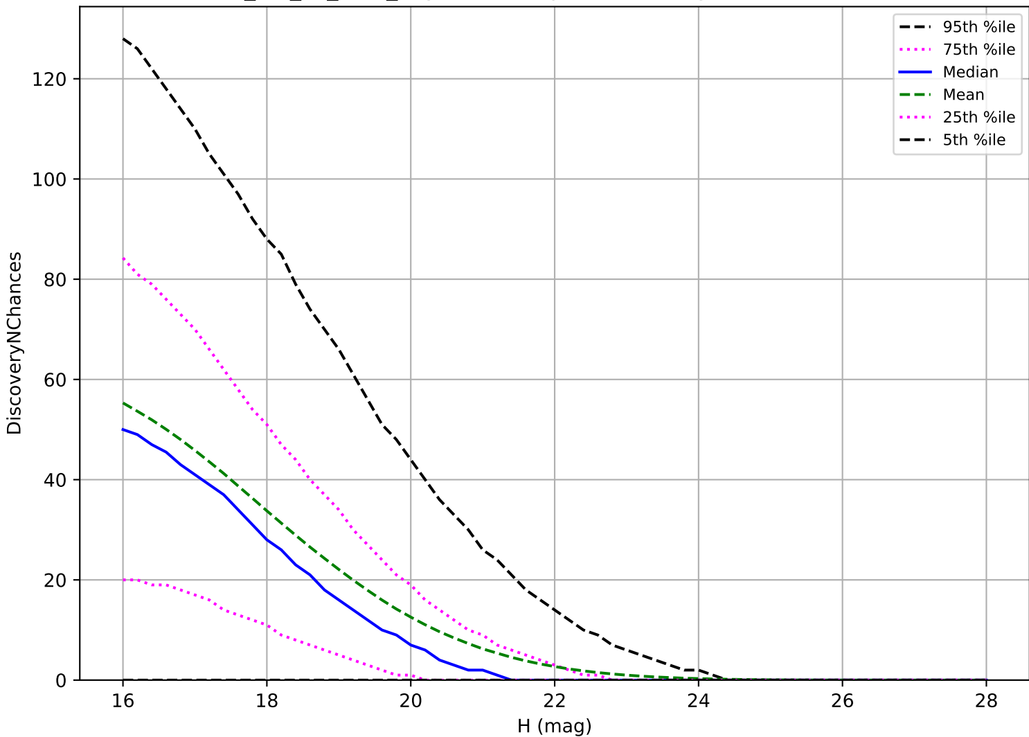
mw_roll_all_v3.3_10yrs: NEO 3 pairs in 15 nights detection loss
