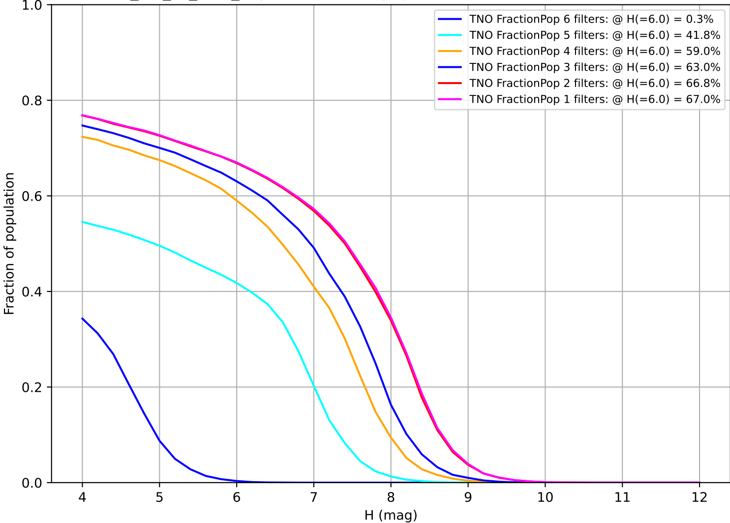
mw_roll_all_v3.3_10yrs: Fraction of population with colors in X filters TNO
