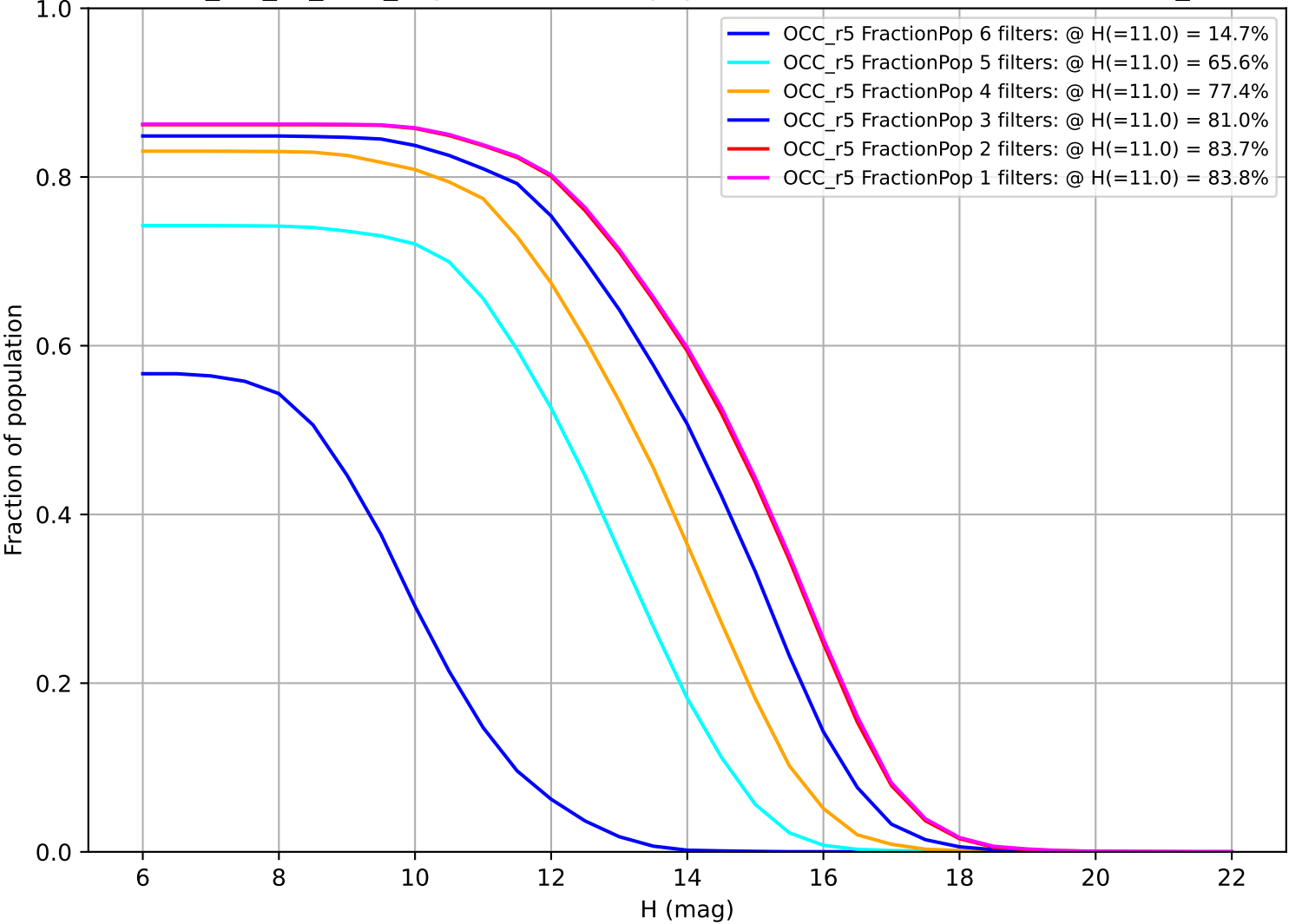
mw_roll_all_v3.3_10yrs: Fraction of population with colors in X filters OCC_r5
