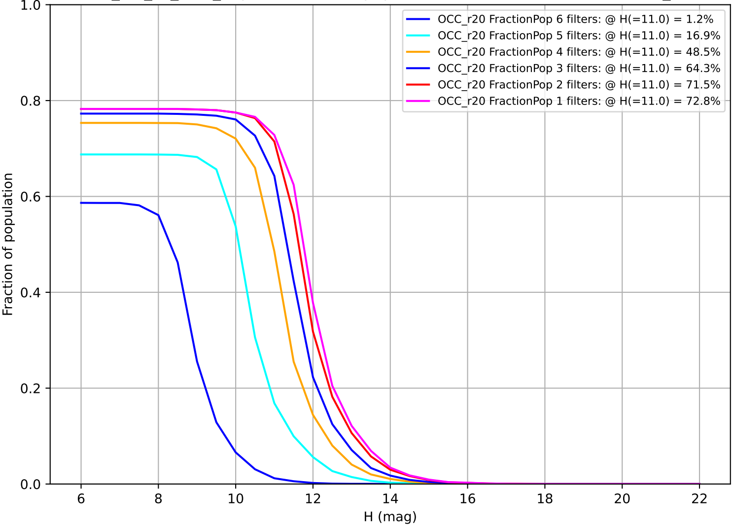
mw_roll_all_v3.3_10yrs: Fraction of population with colors in X filters OCC_r20
