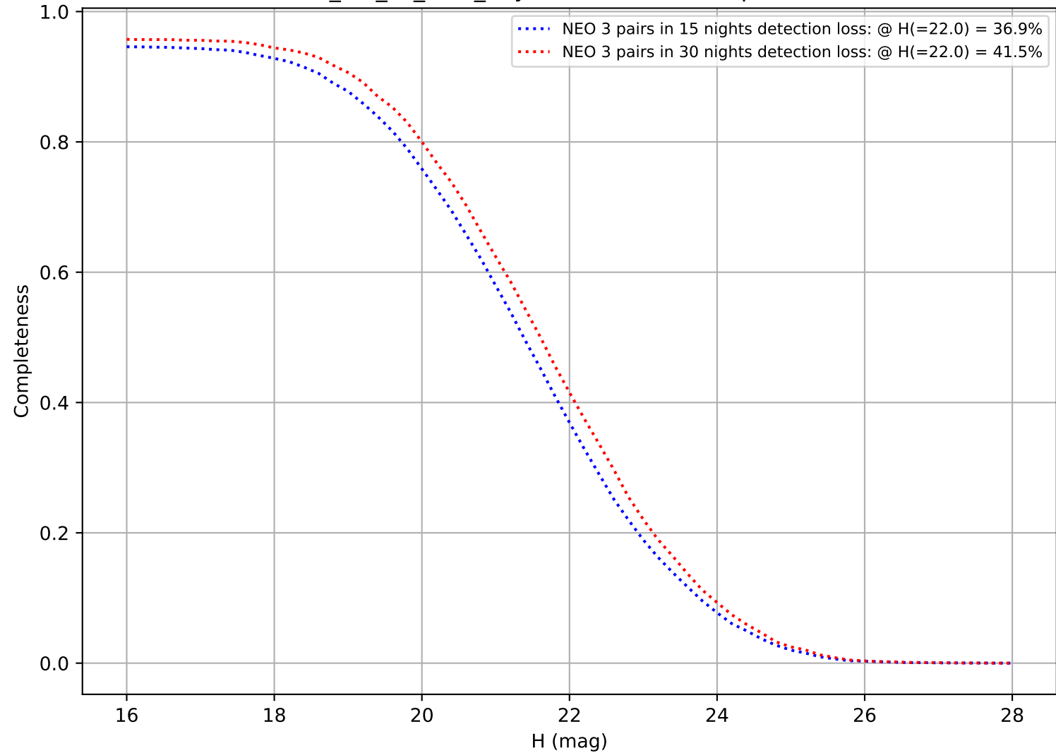
mw_roll_all_v3.3_10yrs: DifferentialCompleteness
