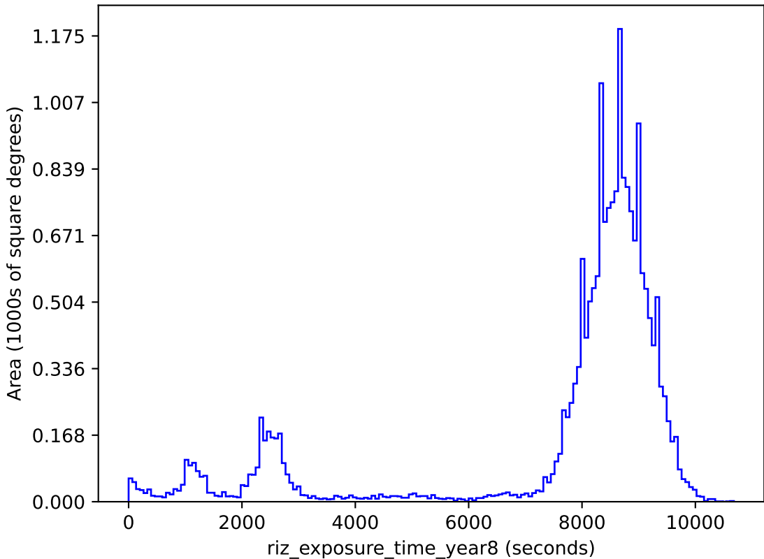
mw_roll_all_v3.3_10yrs gri band non-DD: riz_exposure_time_year8
