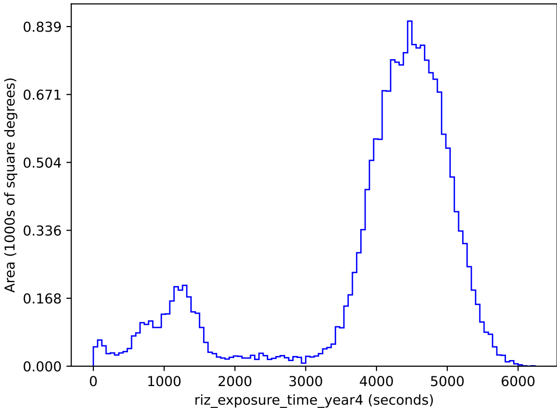
mw_roll_all_v3.3_10yrs gri band non-DD: riz_exposure_time_year4
