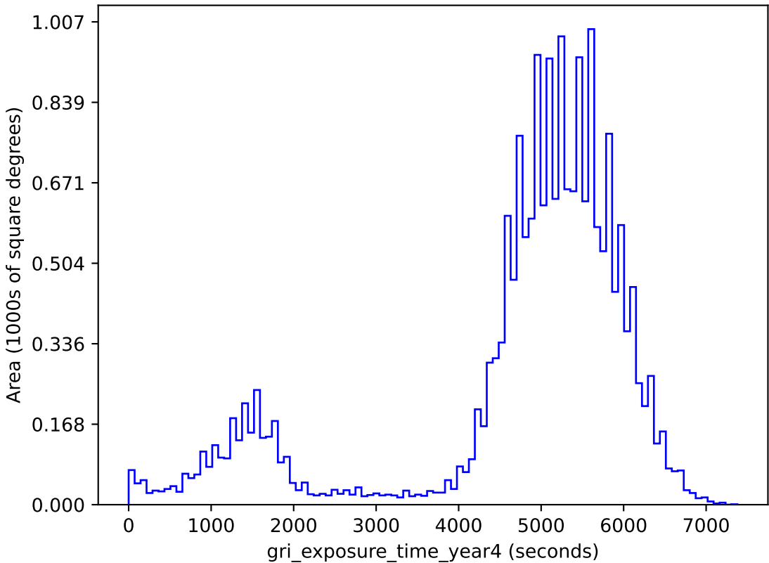
mw_roll_all_v3.3_10yrs gri band non-DD: gri_exposure_time_year4
