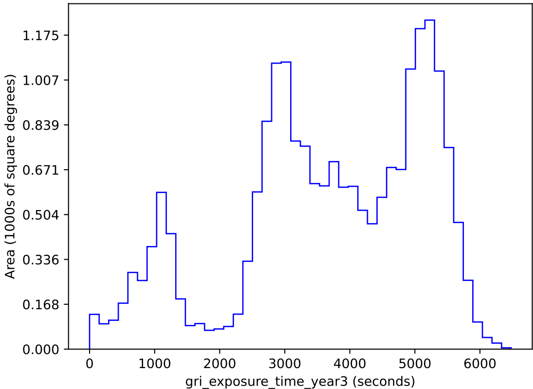
mw_roll_all_v3.3_10yrs gri band non-DD: gri_exposure_time_year3
