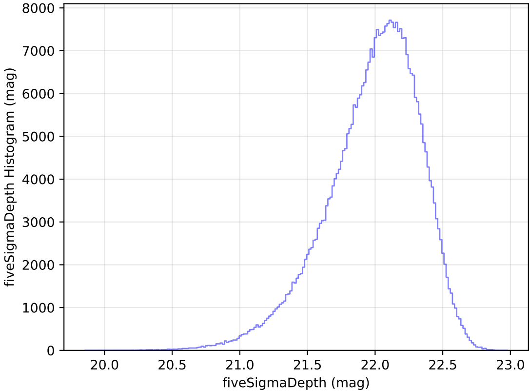
mw_roll_all_v3.3_10yrs y: fiveSigmaDepth Histogram
