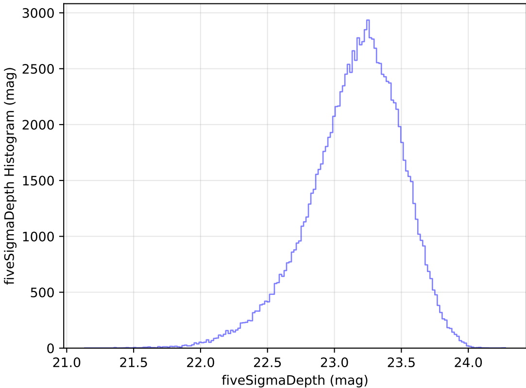
mw_roll_all_v3.3_10yrs u: fiveSigmaDepth Histogram
