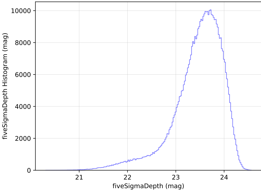
mw_roll_all_v3.3_10yrs i: fiveSigmaDepth Histogram
