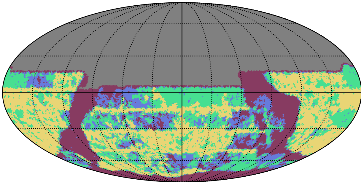
mw_roll_all_v3.3_10yrs u band: YearCoverage night
