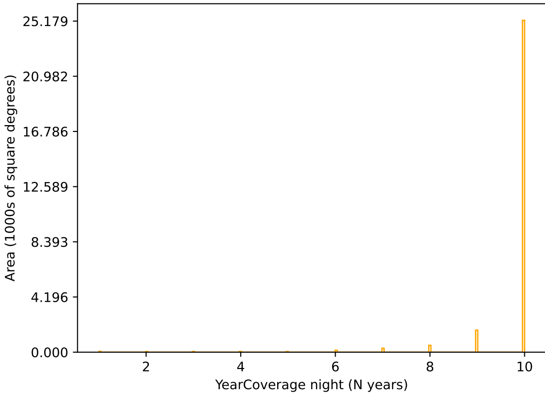
mw_roll_all_v3.3_10yrs r band: YearCoverage night
