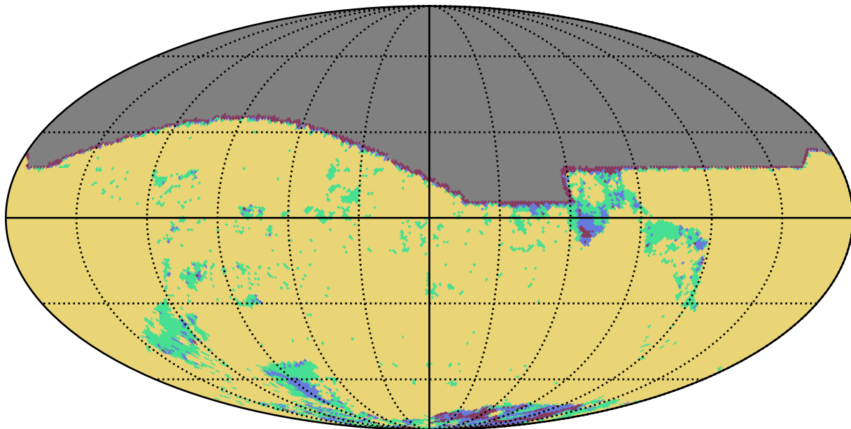
mw_roll_all_v3.3_10yrs i band: YearCoverage night
