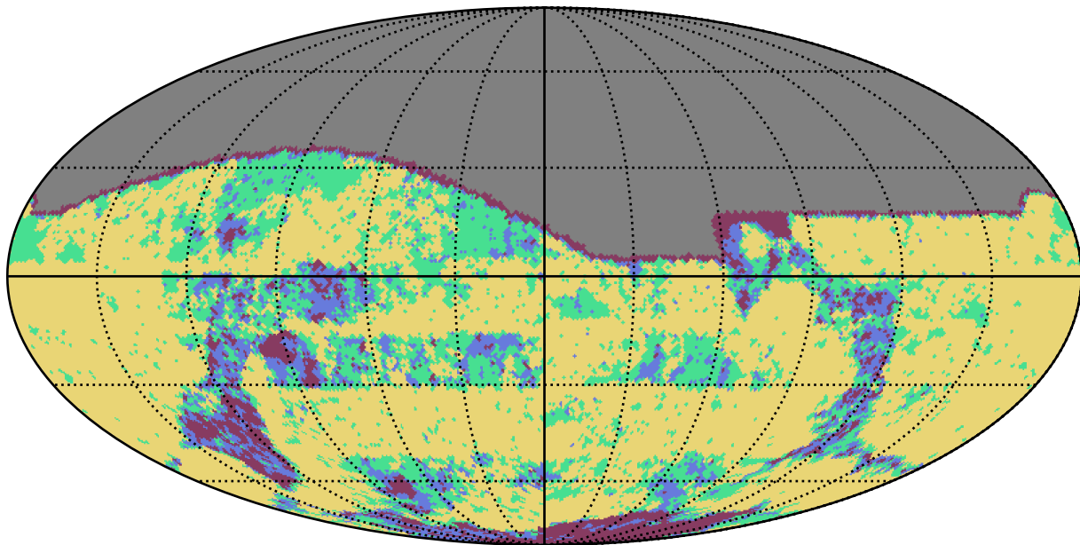
mw_roll_all_v3.3_10yrs g band: YearCoverage night
