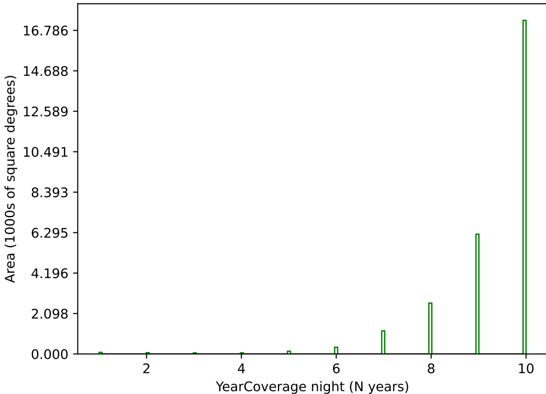
mw_roll_all_v3.3_10yrs g band: YearCoverage night
