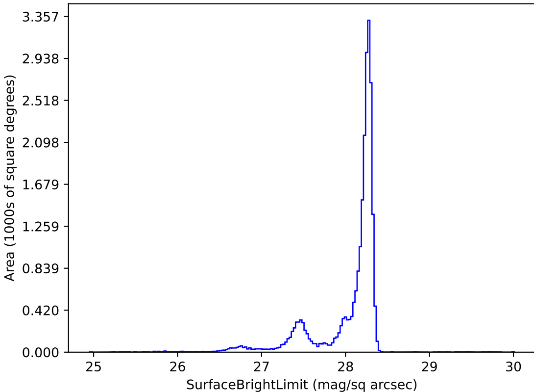
mw_roll_all_v3.3_10yrs y: SurfaceBrightLimit
