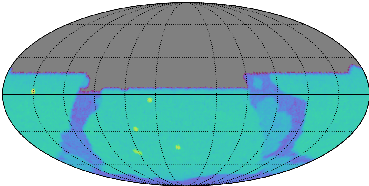
mw_roll_all_v3.3_10yrs u: SurfaceBrightLimit
