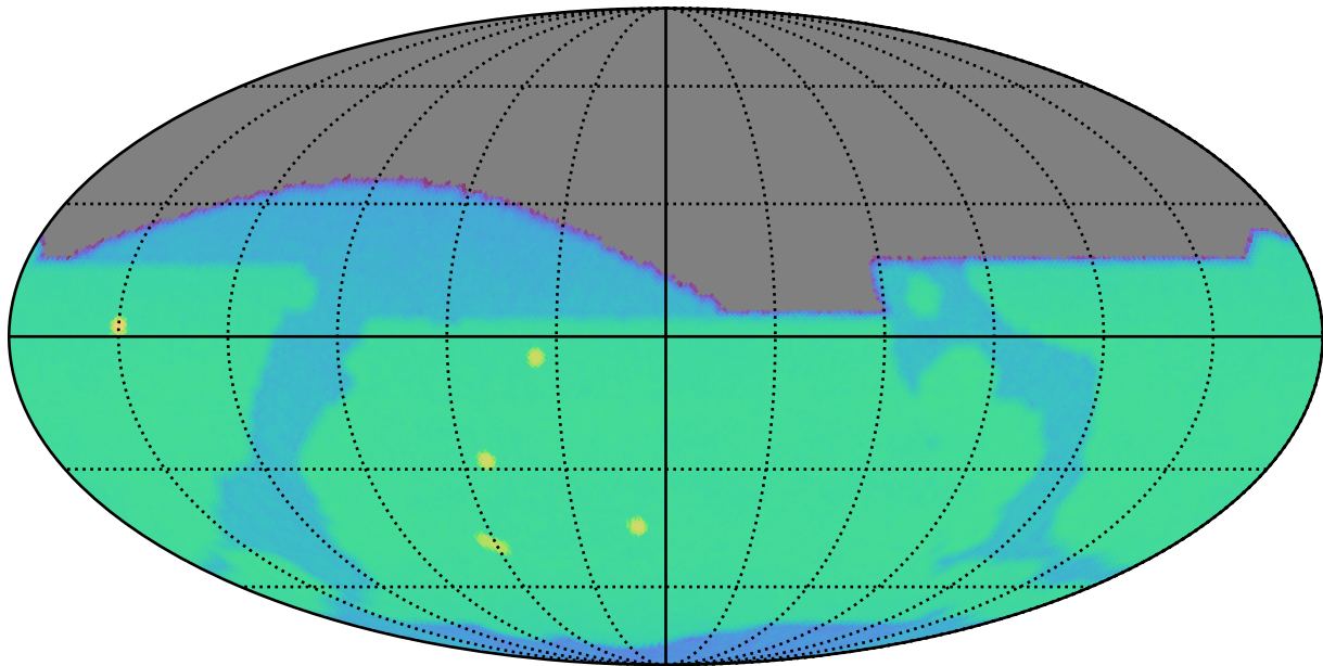
mw_roll_all_v3.3_10yrs i: SurfaceBrightLimit
