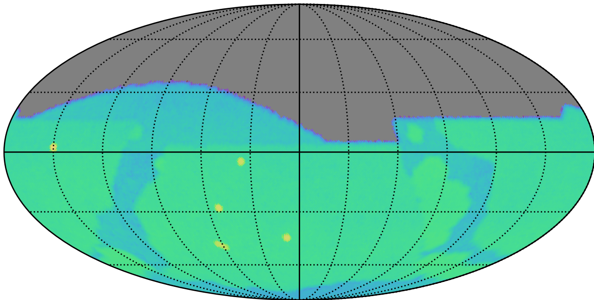
mw_roll_all_v3.3_10yrs g: SurfaceBrightLimit
