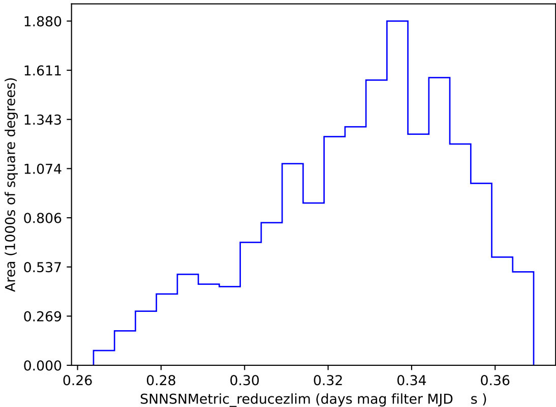
mw_roll_all_v3.3_10yrs DDF excluded: SNNSNMetric_reducezlim
