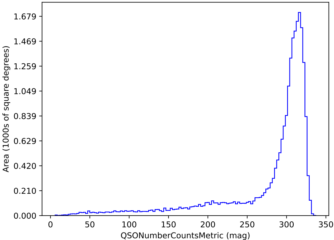
mw_roll_all_v3.3_10yrs u band and non-DD: QSONumberCountsMetric
