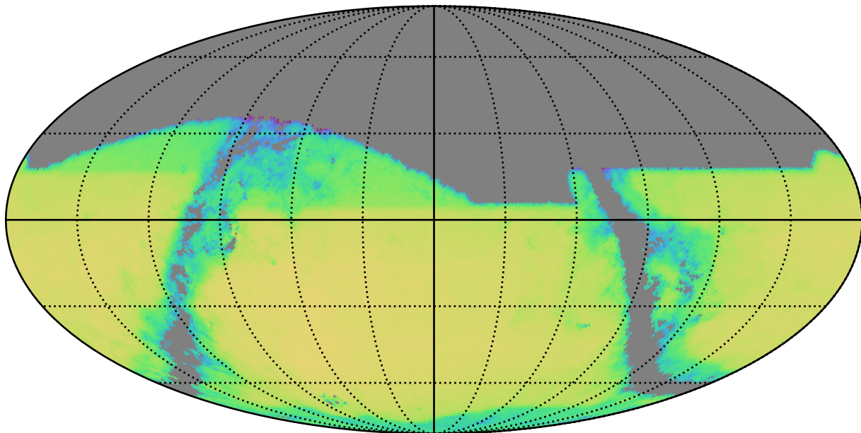
mw_roll_all_v3.3_10yrs r band and non-DD: QSONumberCountsMetric
