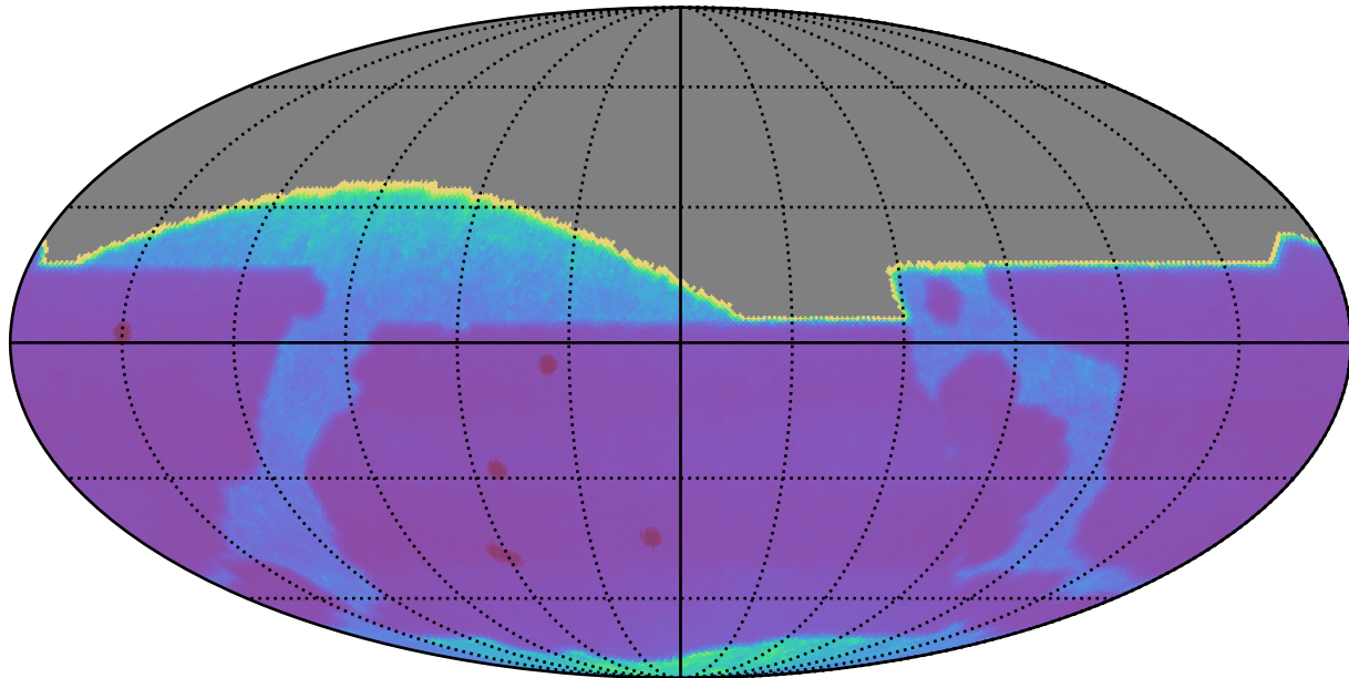
mw_roll_all_v3.3_10yrs : Proper Motion Uncert @ 20.5
