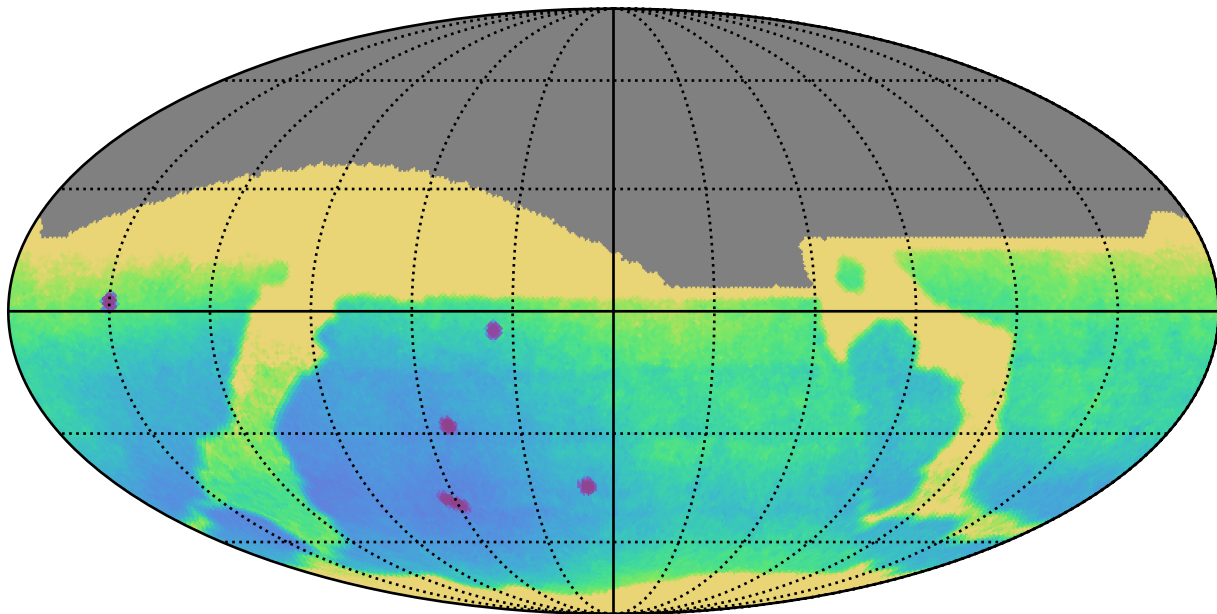
mw_roll_all_v3.3_10yrs : Parallax Uncert @ 24.0
