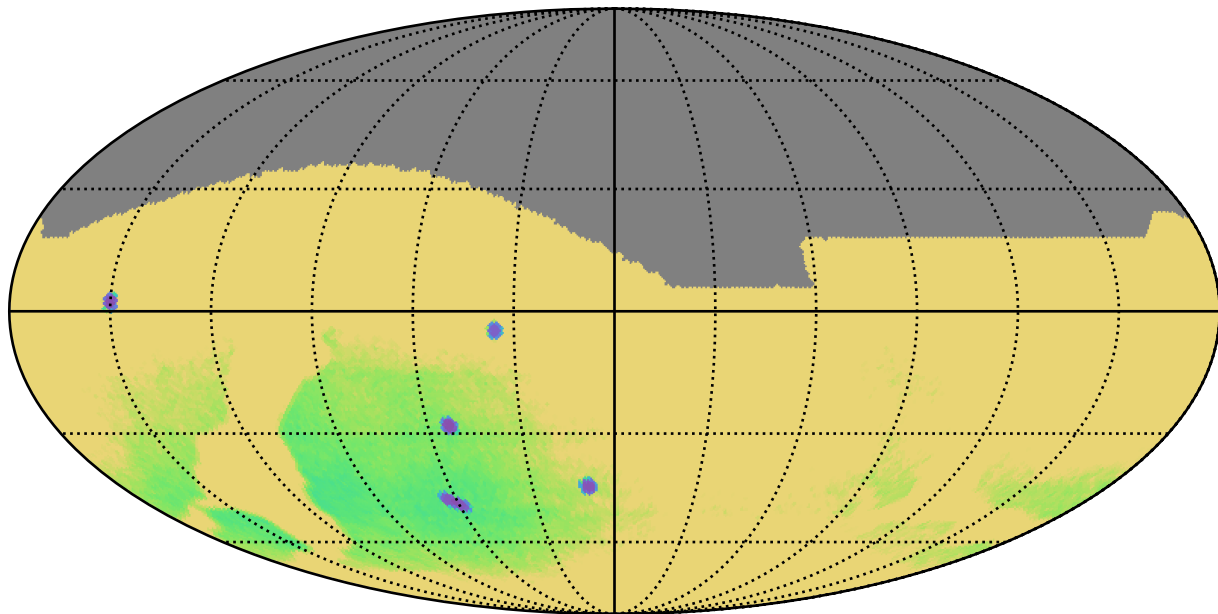
mw_roll_all_v3.3_10yrs : Parallax Uncert @ 22.4
